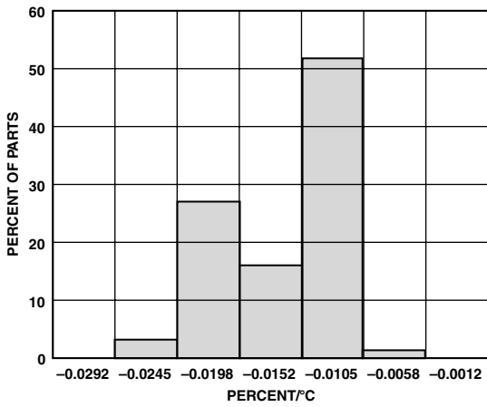
TPC 20. X-Axis Sensitivity Drift at X_{FILTER} Due to Temperature Distribution, -40°C to +85°C
