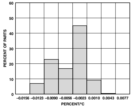
TPC 23. Y-Axis Sensitivity Drift at X_{FILTER} Due to Temperature Distribution, -40°C to +85°C
